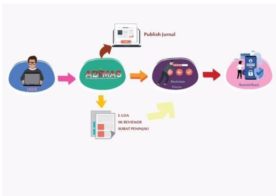
Figure 9. Blockchain workflow
